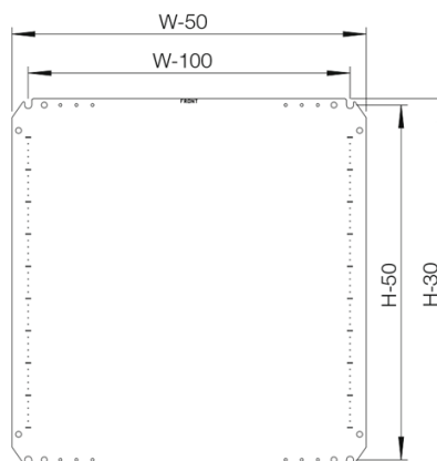
Mounting plate
