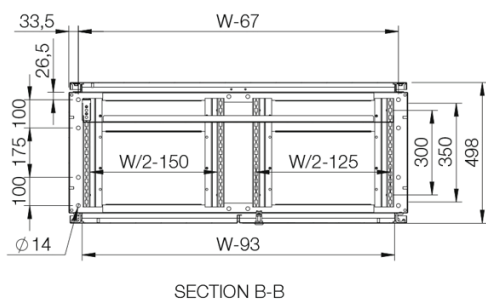
Sectional top view
