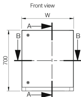
Single door
