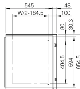
Inside left door view
